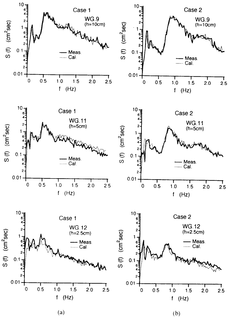
Fig. 5 Comparison between Measured Spectra and Calculated Ones by Hybrid Model Equation.
