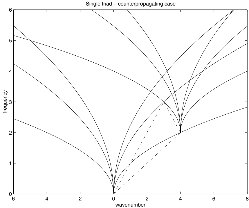
Figure 2: Resonant triad edge-wave interaction with counterpropagating components.
