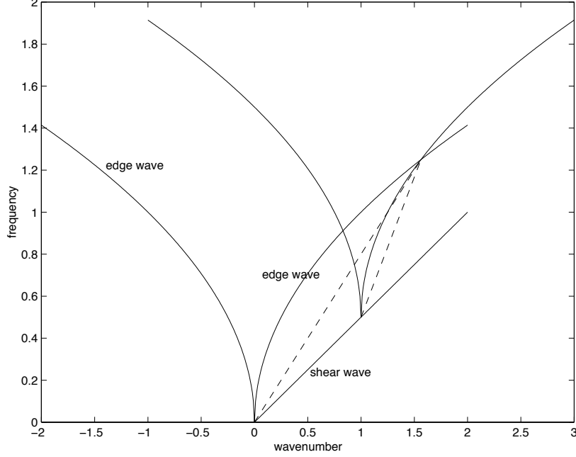
Figure 1: Diagram illustrating hypothetical resonant triad interaction involving a shear wave and two edge waves. Identifying the shear wave as the first wave in the triad, the origin of the edge wave dispersion curve is translated up the shear wave dispersion curve to the locus of shear wave frequency and wavenumber. Resonances involving two edge waves are then indicated by the intersections of the original and the translated edge wave dispersion curves. The two dashed lines here indicate two edge waves with the same mode number and propagating downstream with the longshore current.
