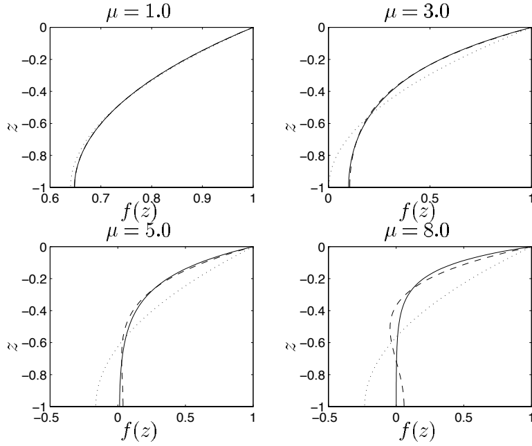
Figure 3: Normalized vertical profile of linear horizontal kinematics for (a) \mu = 1 , (b) \mu = 3 , (c) \mu = 5 , (d) \mu = 8 . Exact (solid), Nwogu (dotted), Present (dash)
