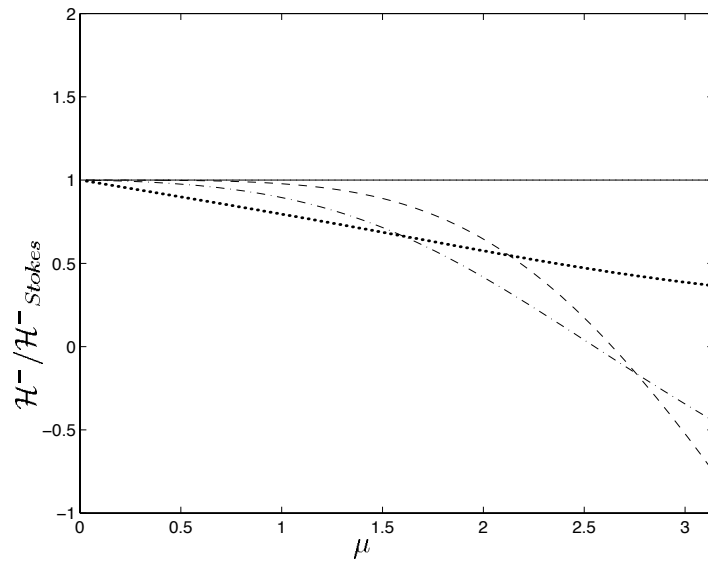
Figure 7: Ratio of approximate subharmonic transfer coefficients to Stokes' solution. Stokes' theory (solid), Nwogu (dotted), WKGS (dash-dot), Present (dash), Present rearranged (thin dot)
