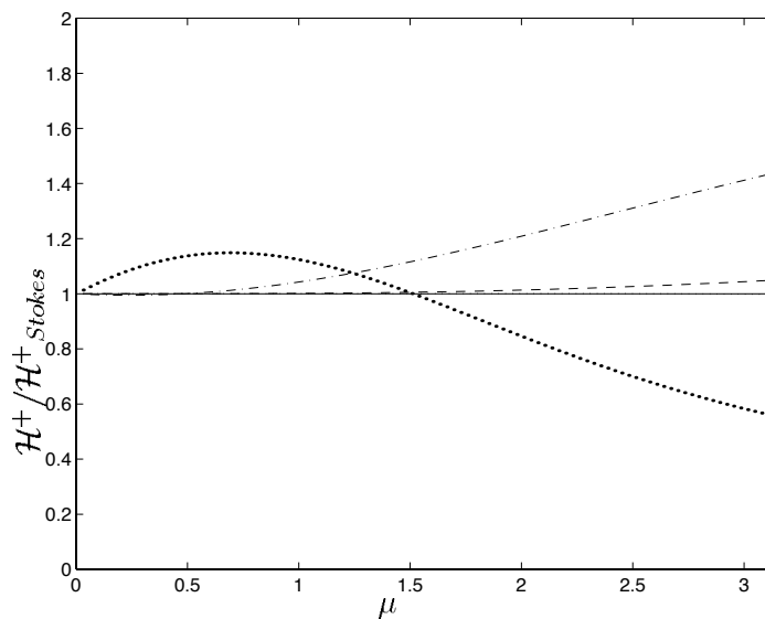
Figure 6: Ratio of approximate superharmonic transfer coefficients to Stokes' solution. Stokes' theory (solid), Nwogu (dotted), WKGS (dash-dot), Present (dash), Present rearranged (thin dot)
