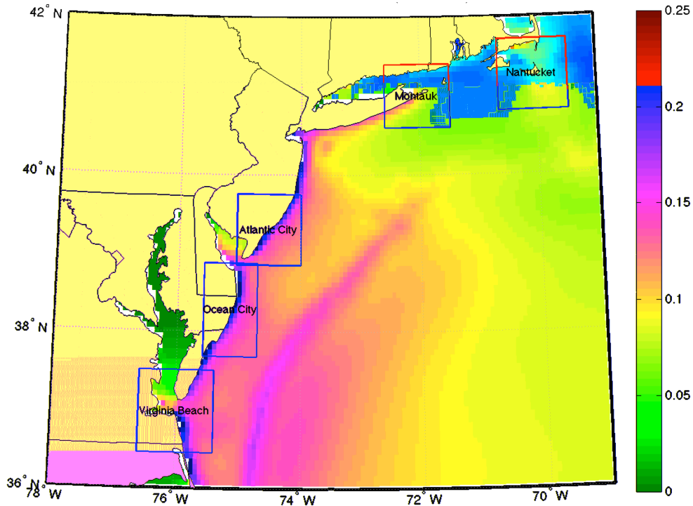
Fig. 13: Envelope of maximum surface elevation (in m) for AGCZ sources (see Fig. 2): (a) 35.144N and -10.055W source (lower source in Fig. 2) in 4' grid; (b) same source in 2' grid; (c) for all the AGCZ sources, in 2' grid.
