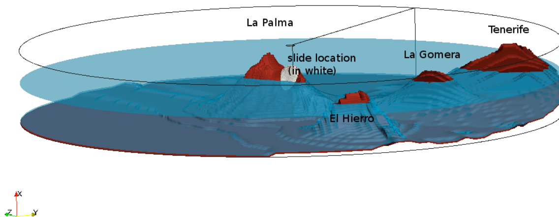
Fig. 5: Sketch of cylindrical computational domain in THETIS model, for CVV flank collapse simulations, assuming a 80 km 3 subaerial slide case, with view of bottom bathymetry, neighboring islands, and slide location (marked in white) (Abadie et al., 2011, 2012).
