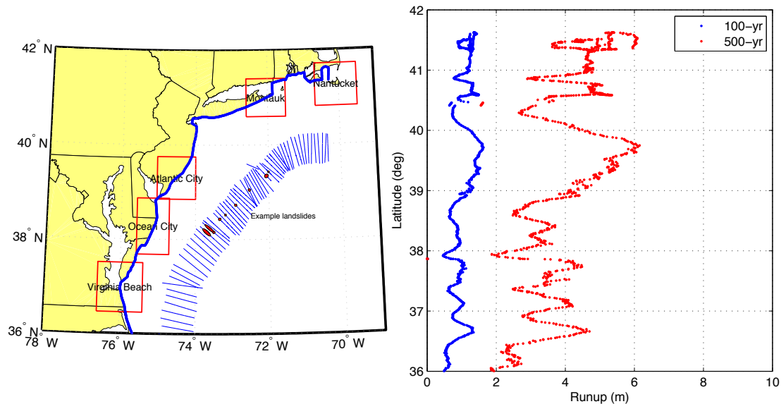
Fig. 7: Right panel: 100-yr and 500-yr runup predictions. Left panel: SMF transects (blue lines) used in MC analysis and location and size of underwater landslides causing 500 year runup (red ellipses). The solid blue line indicates the simplified coastline used in MC simulations and the red boxes mark the size and locations of DEMs currently available from NOAA-NGDC.
