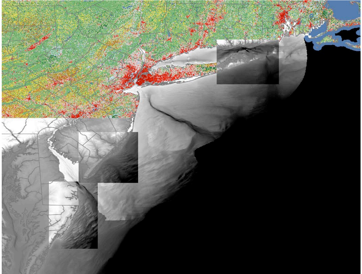
Figure 2: Mosaic of DEM and land use information based on NGDC tsunami DEM's, FEMA DEM's for Region 2 and Region 3 hurricane studies, and National Land Cover Data. Work covered by this project will provide maps for the Ocean City, Atlantic City and Montauk DEM's (smallest highlighted areas) and Myrtle Beach, SC using NGDC DEM's, and the remainder of the western half of Long Island using FEMA DEM's.
