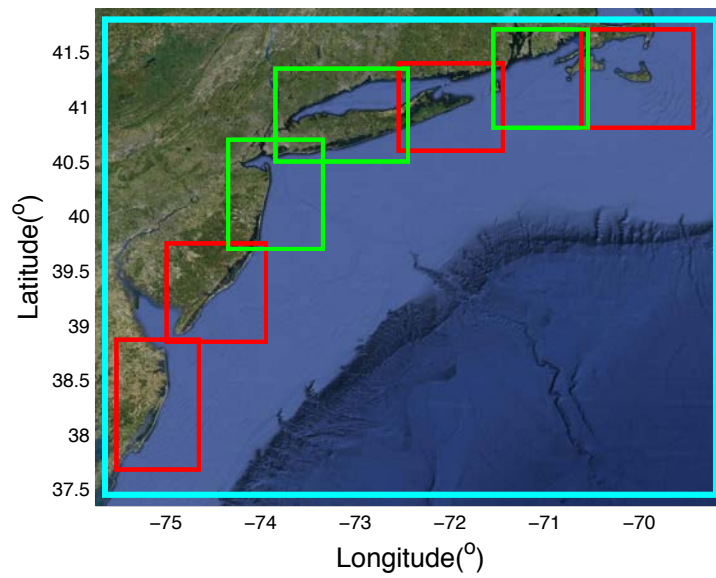
Figure 3: Sequence of DEM's being used for high resolution modeling in N.E. US. Red boxes indicate NGDC tsunami DEM's, including Ocean City, MD, Atlantic City, NJ, Montauk, NY and Martha's Vinyard, MA. Green boxes are similarly sized DEM's developed using FEMA DEM's, providing coverage of Northern New Jersey, New York and Narragansett Bay, Rhode Island.
