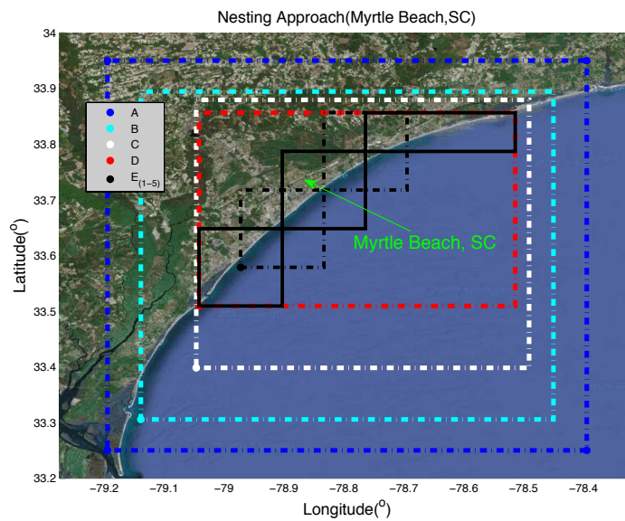
Figure 4: Sequence of nested grids within tsunami DEM's used to get final 10m resolution at inundated shoreline. Myrtle Beach, SC NGDC DEM.
